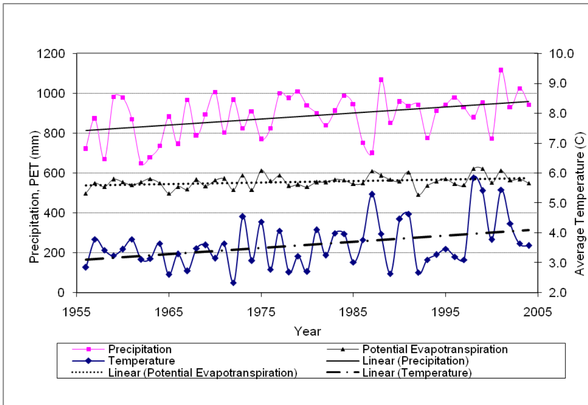
Figure 2.2 – Long term climatic trends at Sudbury Airport (EC, 2002)
